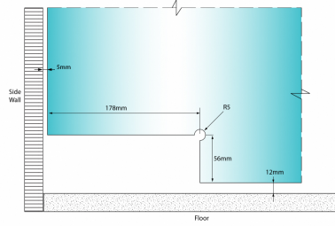
Bottom Patch Cut Out - KGT1055-AUTO100
