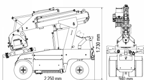
Transport position
