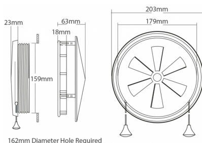
162mm Diameter Hole Required
