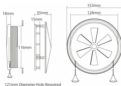
121mm Diameter Hole Required
